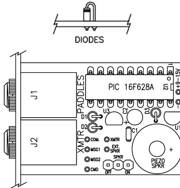
Parts placement figure
